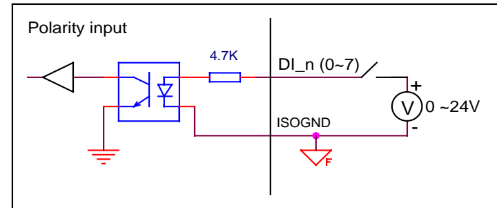
Figure 4-2 isolated digital inputs of PCX-3008
