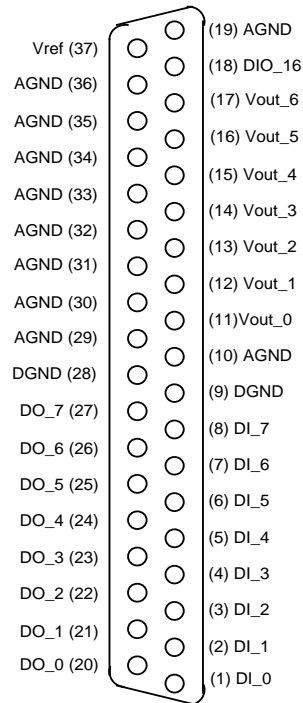
Figure 2-1 Pin Assignment of PCX-3008 connector CN1
