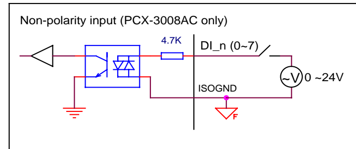
Figure 4-3 isolated digital inputs of PCX-3008AC
